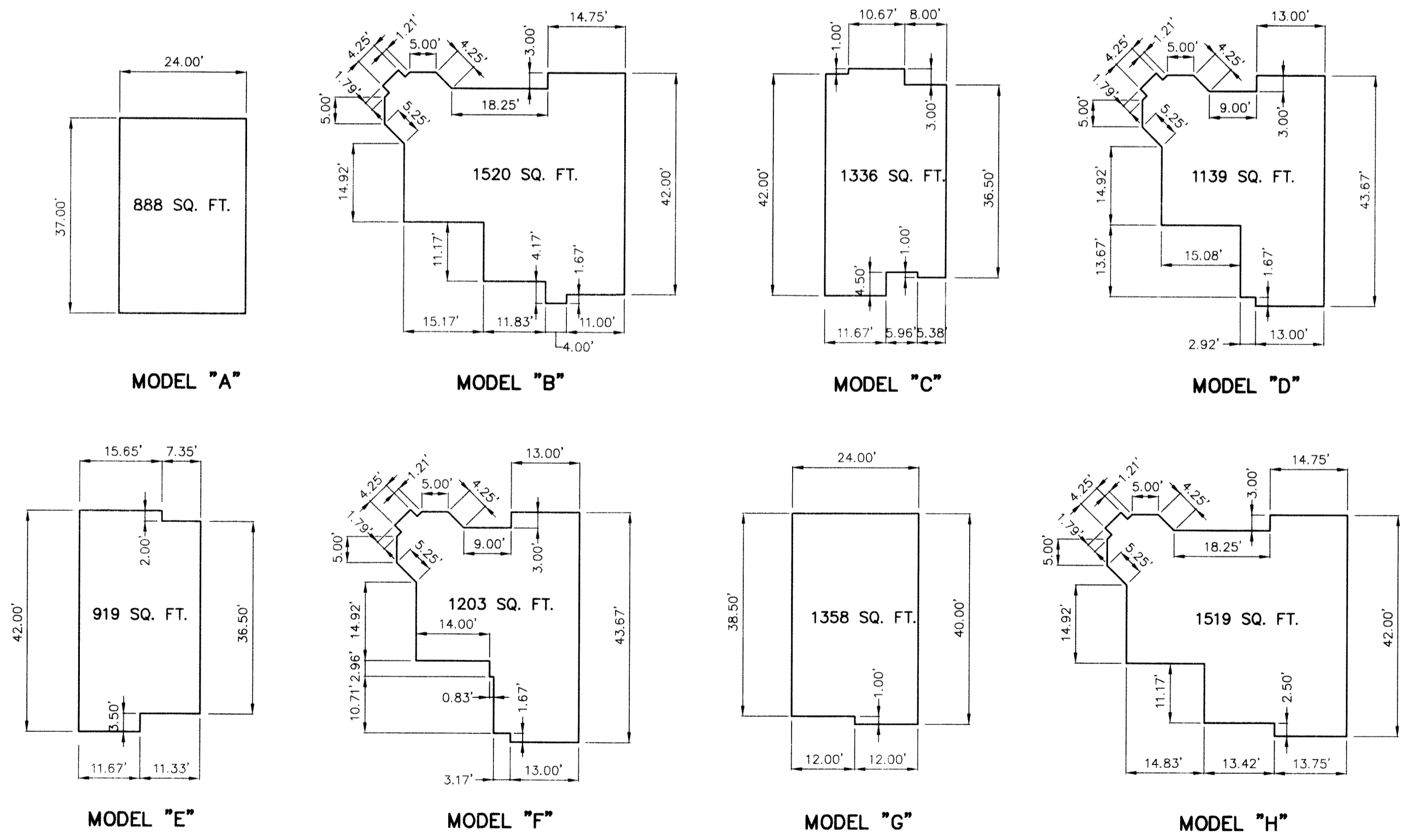
TYPICAL UNIT PLANS 1" = 20'
